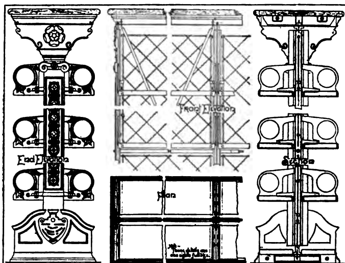
FIG. 40.—Details of Lambert's Adjustable Metal Shelving (Section 181).
